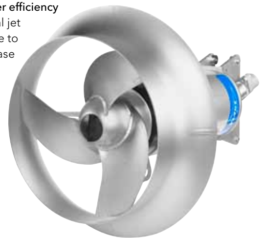
Optional jet ring for increased mixing efficiency.
