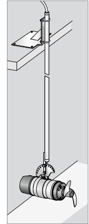
Cantilever mounting Mounts on a cantilever bar, which is fixed to the tank edge.
